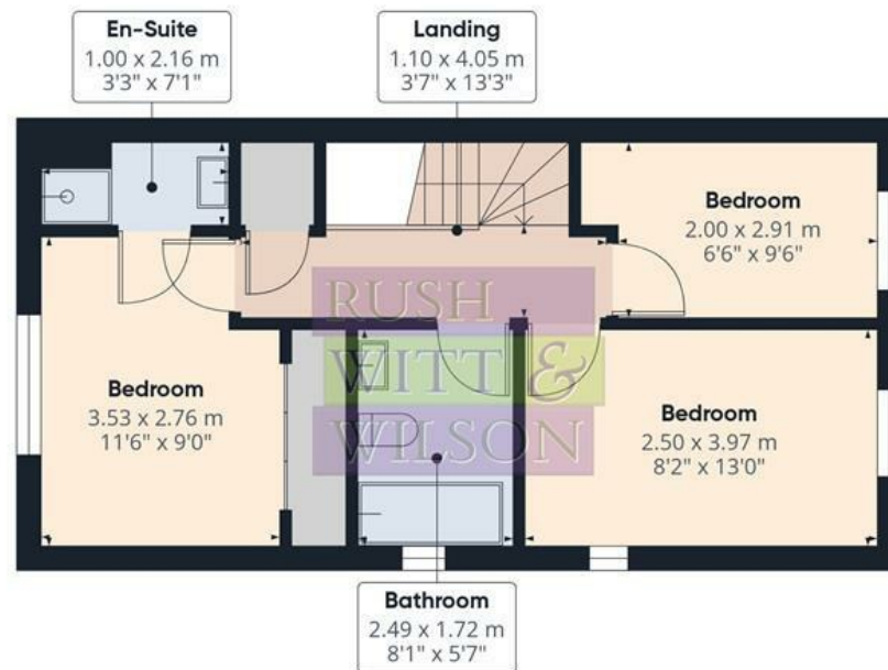
Floor 1 Building 1
